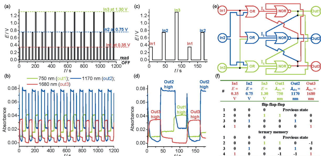
Figure 6. The input (a,c) and output (b,d) signal changes and truth tables (f) of the flip-flop or ternary memory based on the poly-3 3+ /ITO film ( \Gamma = 1.4 \times 10^{-9} mol cm -2 , about 15–20 nm thick). (c) and (d) are partially enlarged plots of (a) and (b), respectively. e) The logic circuit of flip-flop. Ten repeated In1-read-In2-read-In3-read cycles are shown.
